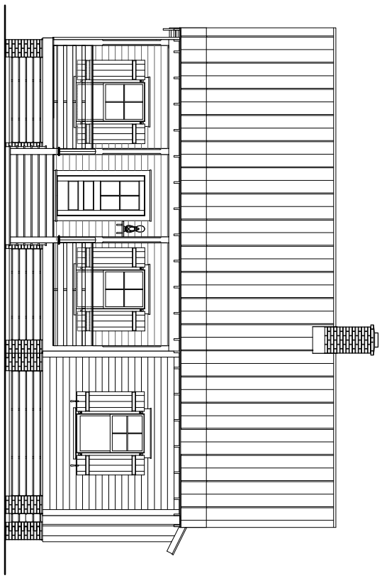
B ALTERNATE FRONT ELEVATION
