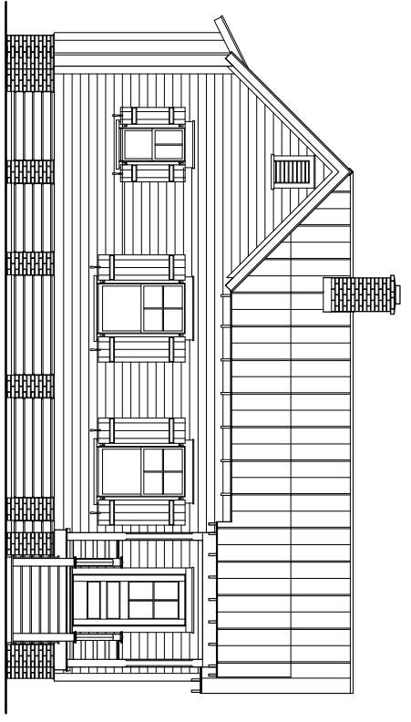
C REAR ELEVATION
