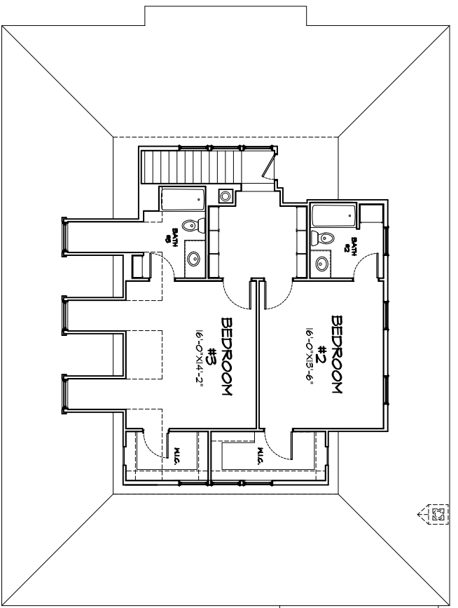
B SECOND FLOOR PLAN
