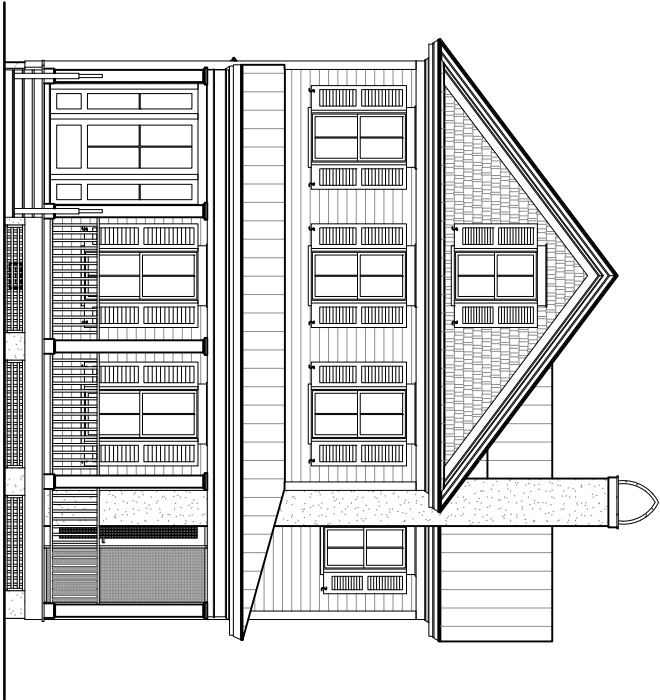
A FRONT ELEVATION
