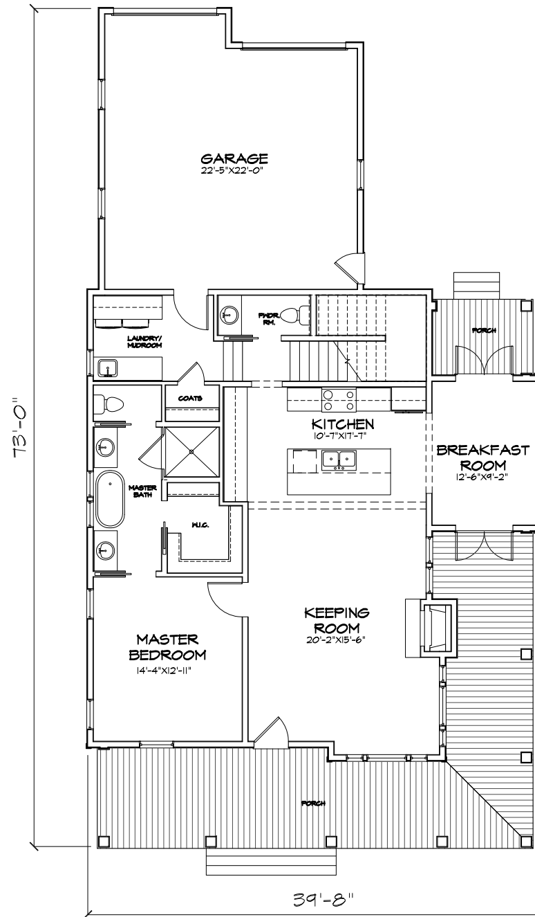
A FIRST FLOOR PLAN
