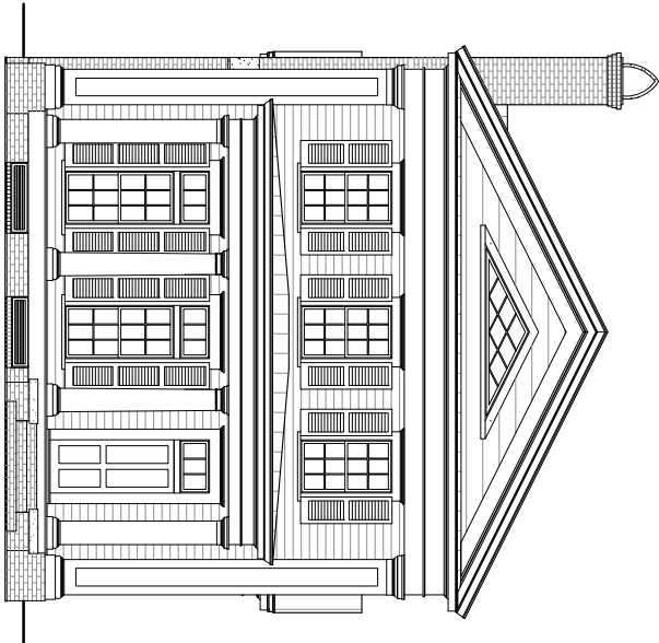
A FRONT ELEVATION NOT TO SCALE
