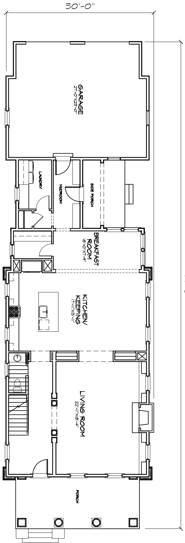
A FIRST FLOOR PLAN
