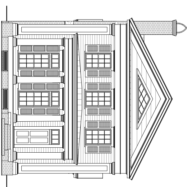
A FRONT ELEVATION NOT TO SCALE
