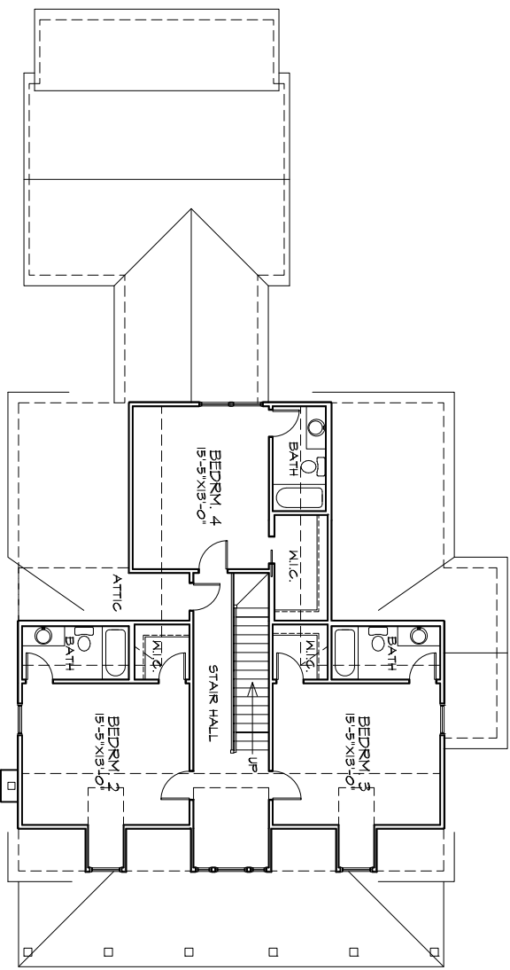
B SECOND FLOOR PLAN
