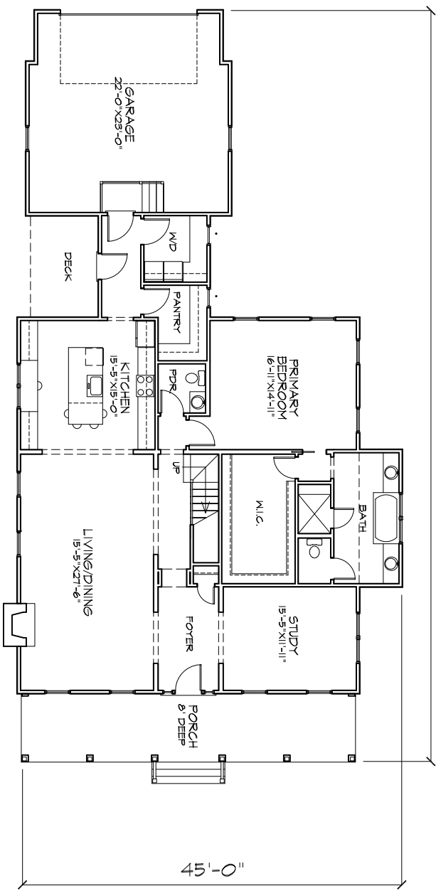
A FIRST FLOOR PLAN
