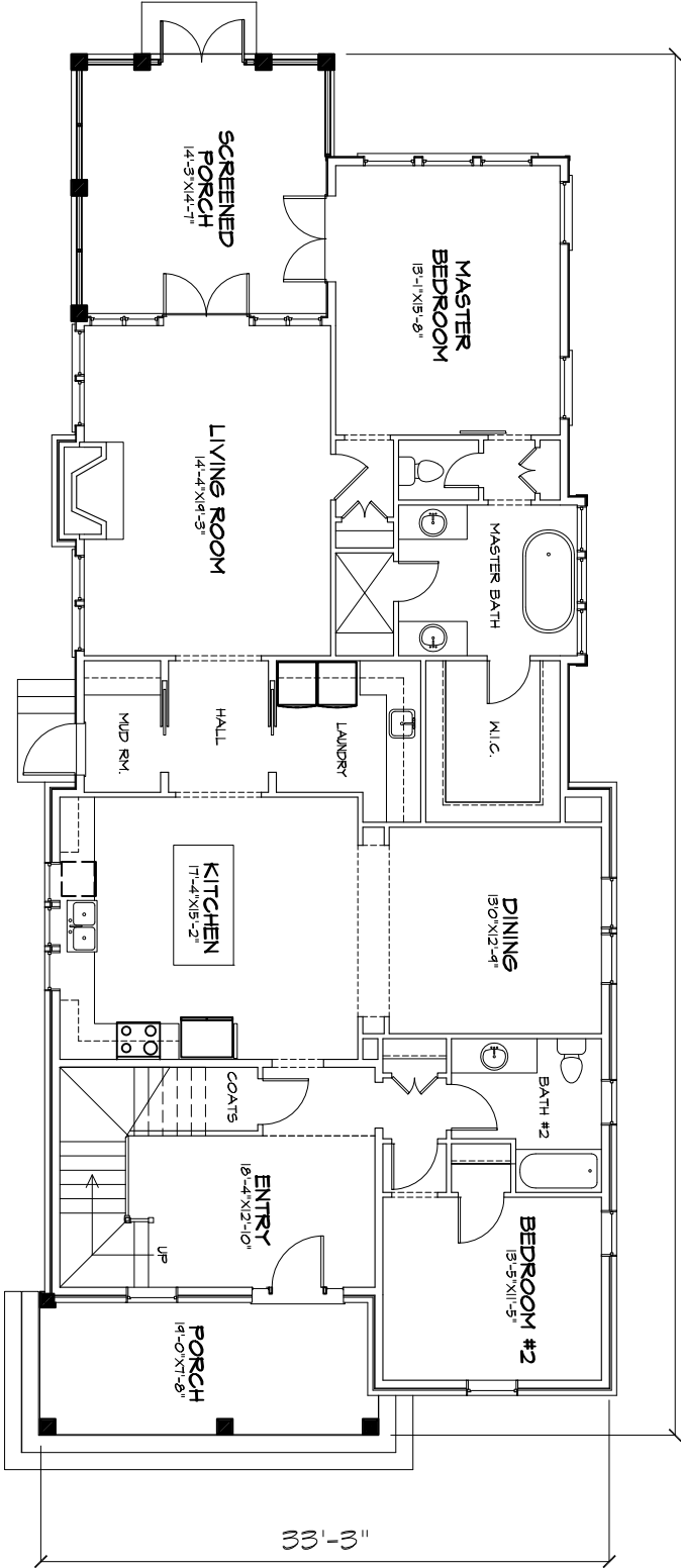
A FIRST FLOOR PLAN
