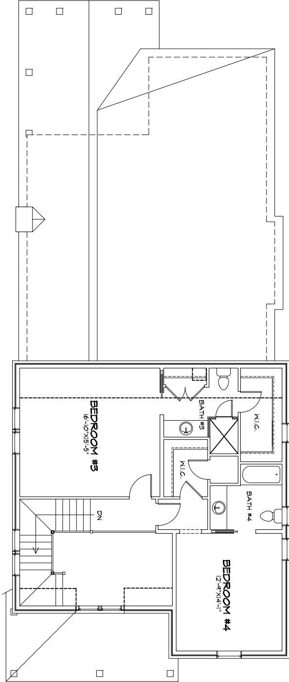
B SECOND FLOOR PLAN
