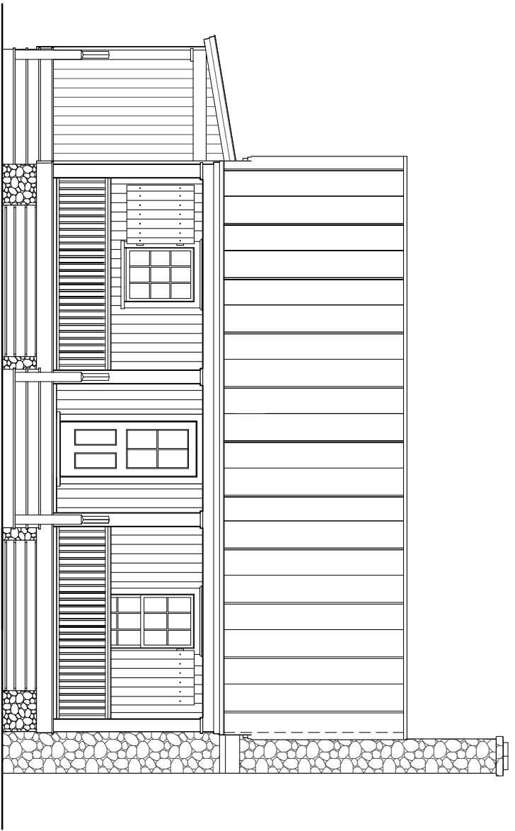
A FRONT ELEVATION
