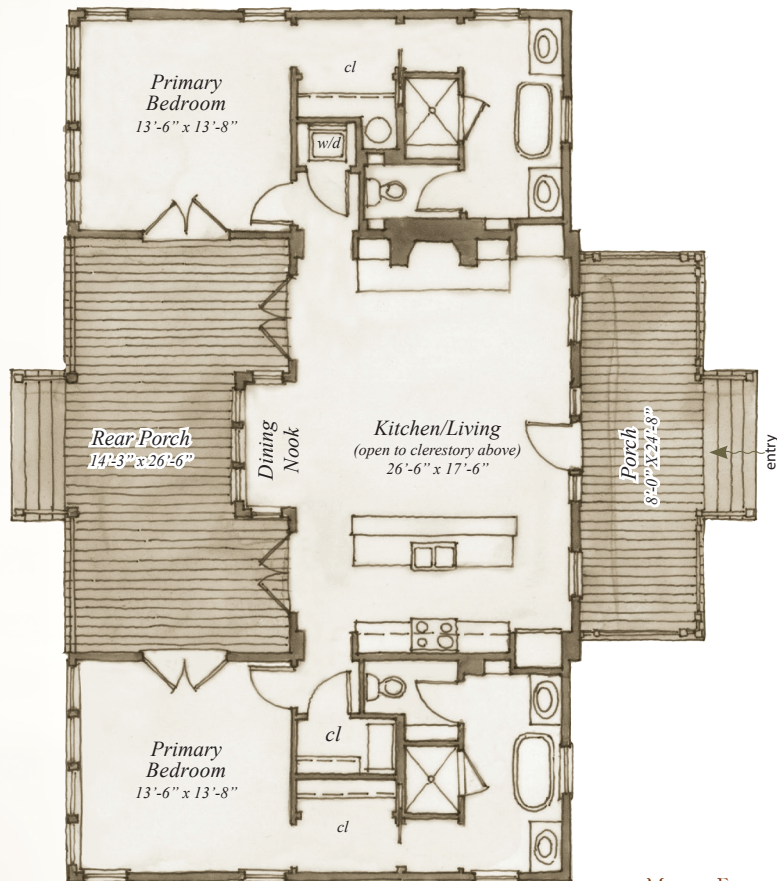
MAIN FLOOR 1,430 S.F.
