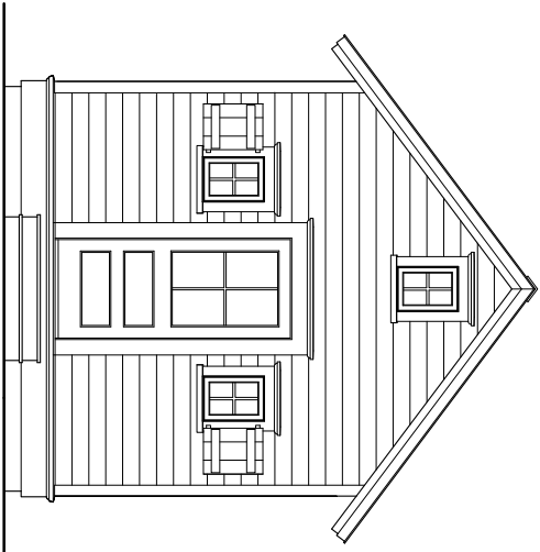
B FRONT ELEVATION
