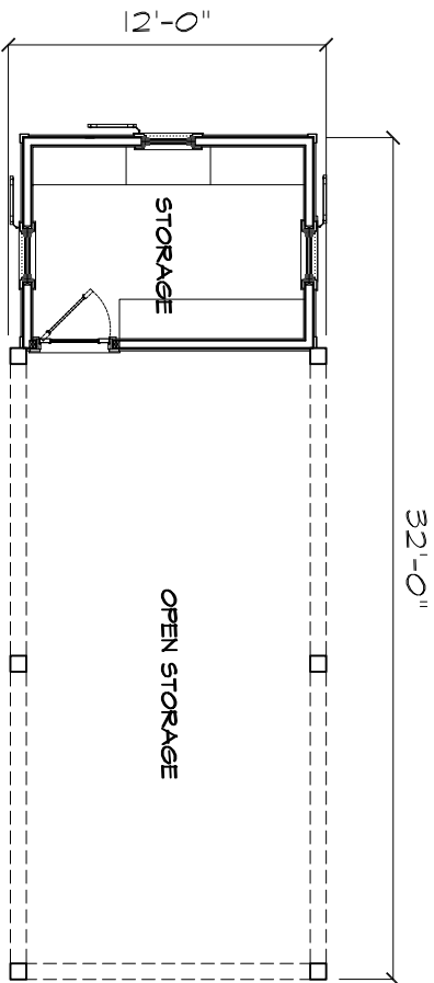
A FLOOR PLAN
