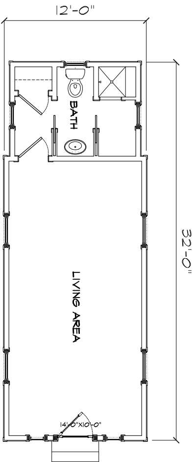
A FLOOR PLAN
