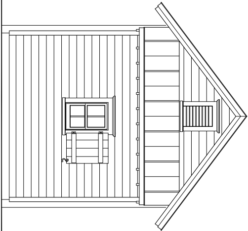
B REAR ELEVATION
