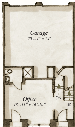
1ST FLOOR 461 S.F.
