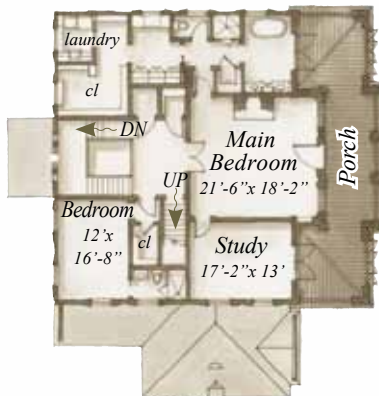
UPPER FLOOR 2021 S.F.
